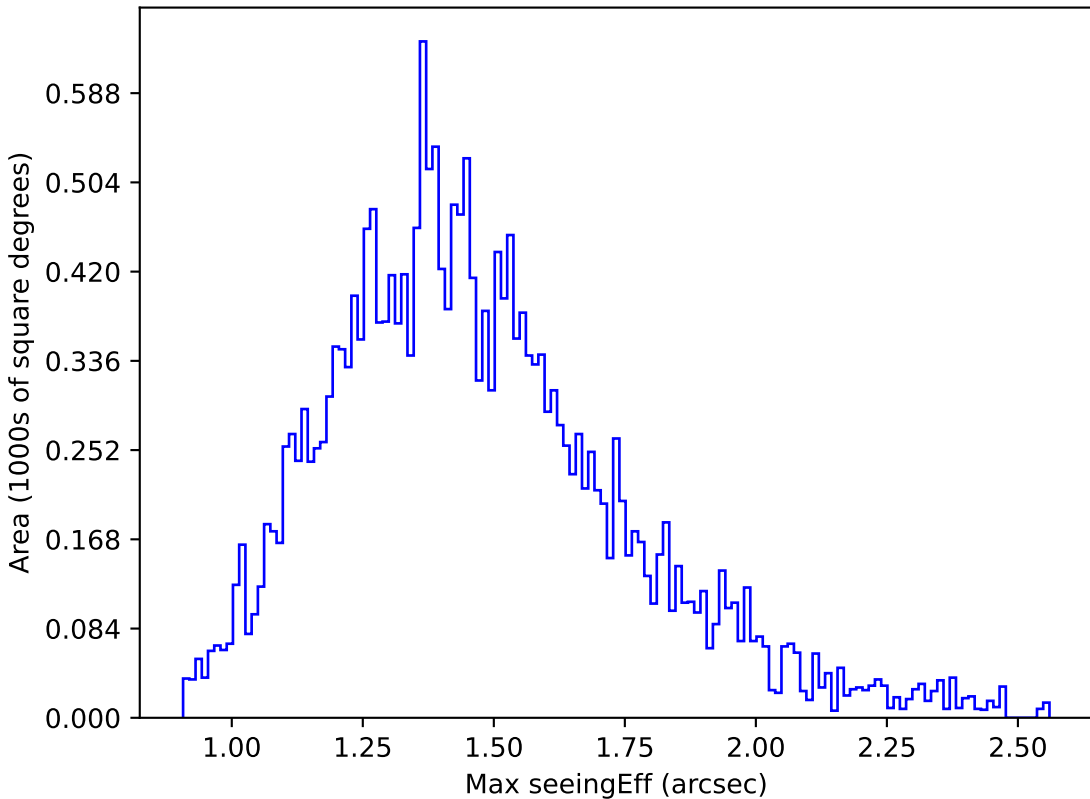
weather_cloudso31v3.4_10yrs Yr 1 y band: Max seeingEff
