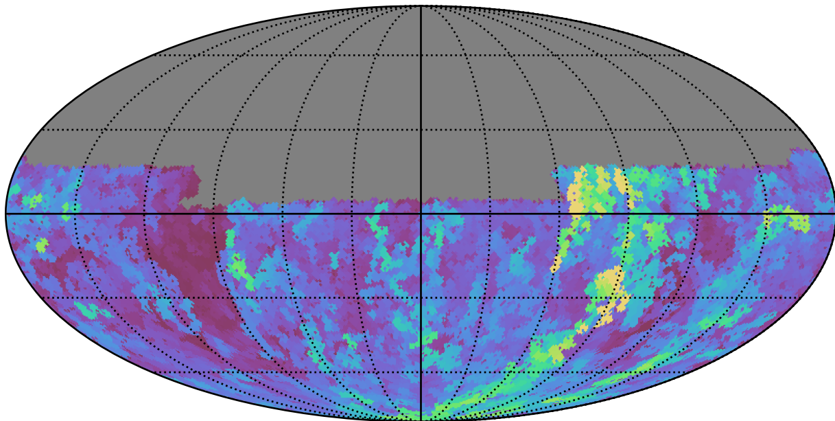
weather_cloudso31v3.4_10yrs Yr 1 u band: Max seeingEff
