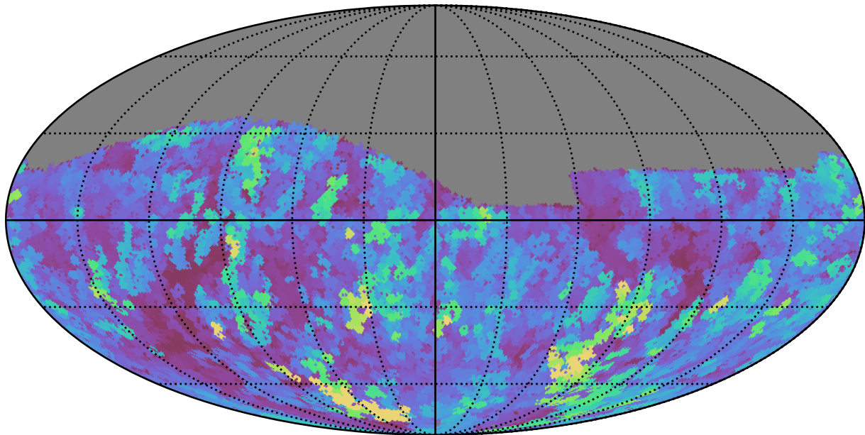
weather_cloudso31v3.4_10yrs Yr 1 r band: Max seeingEff
