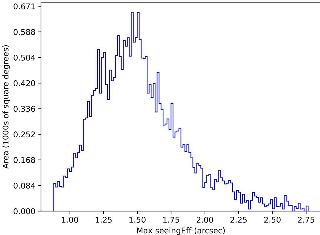
weather_cloudso31v3.4_10yrs Yr 1 r band: Max seeingEff
