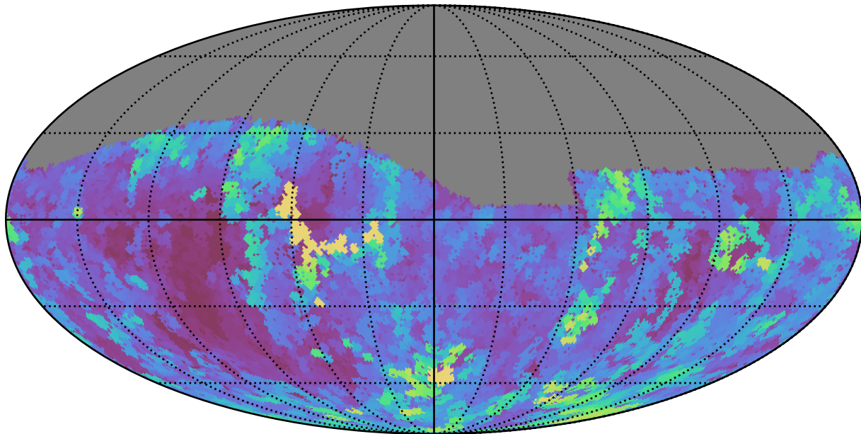
weather_cloudso31v3.4_10yrs Yr 1 g band: Max seeingEff
