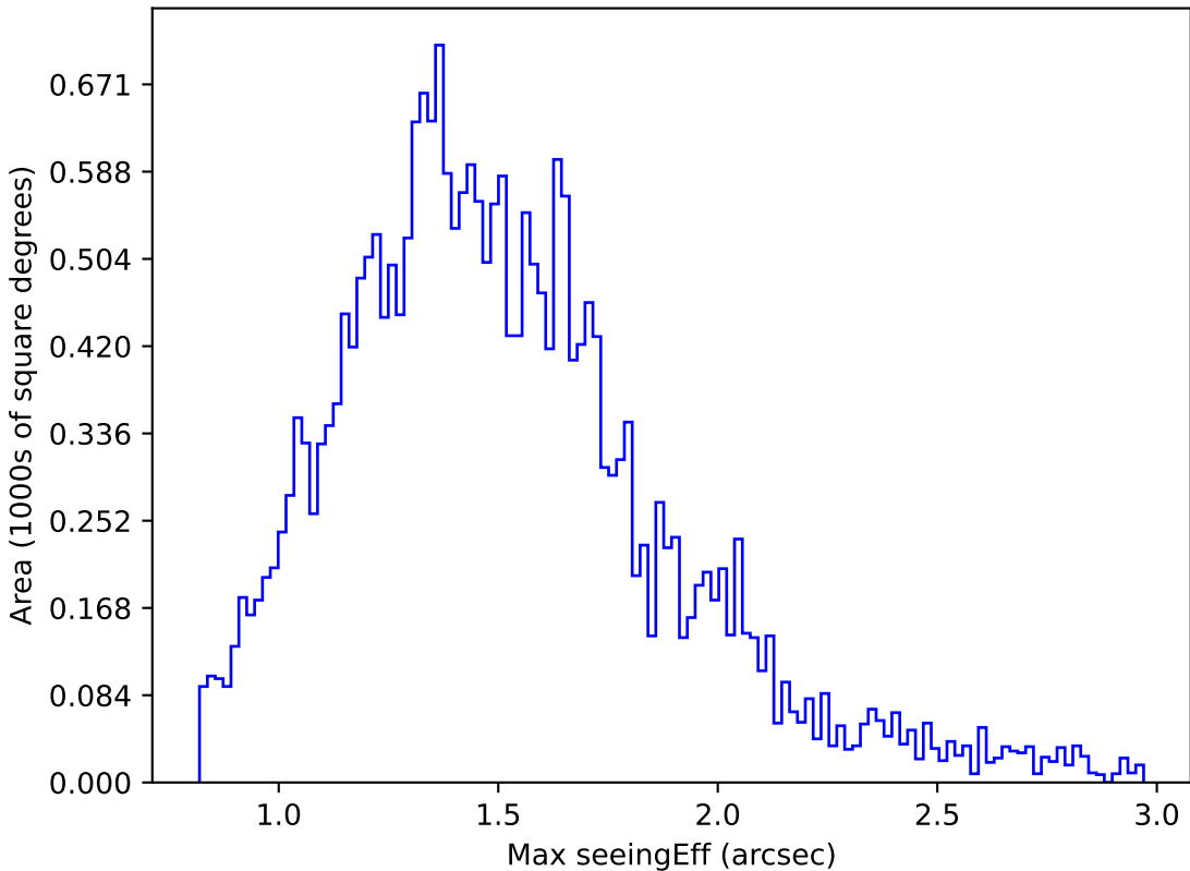
weather_cloudso31v3.4_10yrs Yr 1 g band: Max seeingEff
