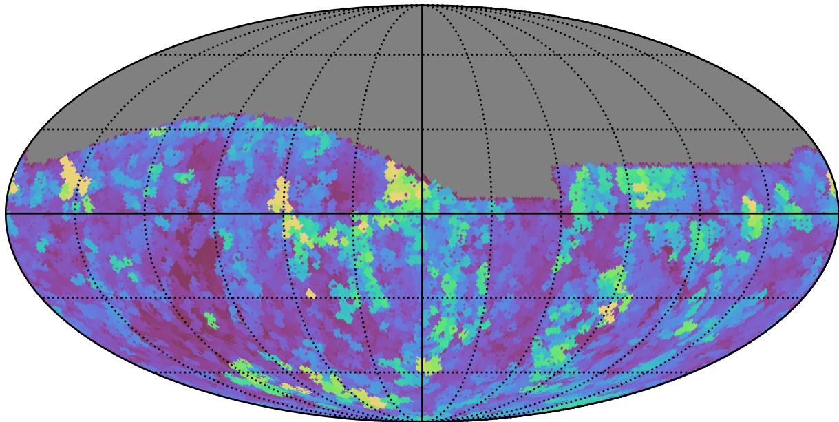
weather_cloudso31v3.4_10yrs Yr 1 all bands: Max seeingEff
