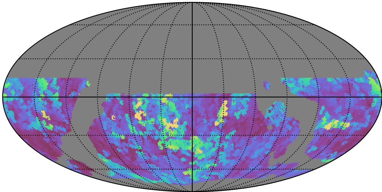
weather_cloudso31v3.4_10yrs WFD z band: Max seeingEff
