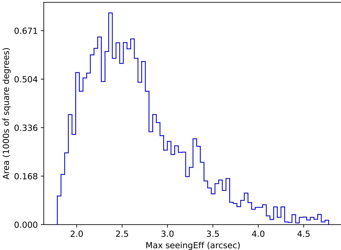
weather_cloudso31v3.4_10yrs WFD z band: Max seeingEff
