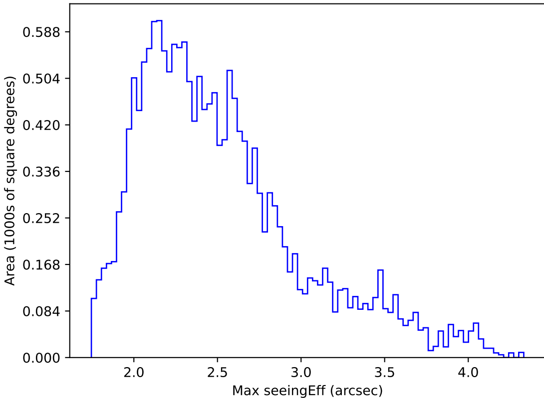
weather_cloudso31v3.4_10yrs WFD y band: Max seeingEff
