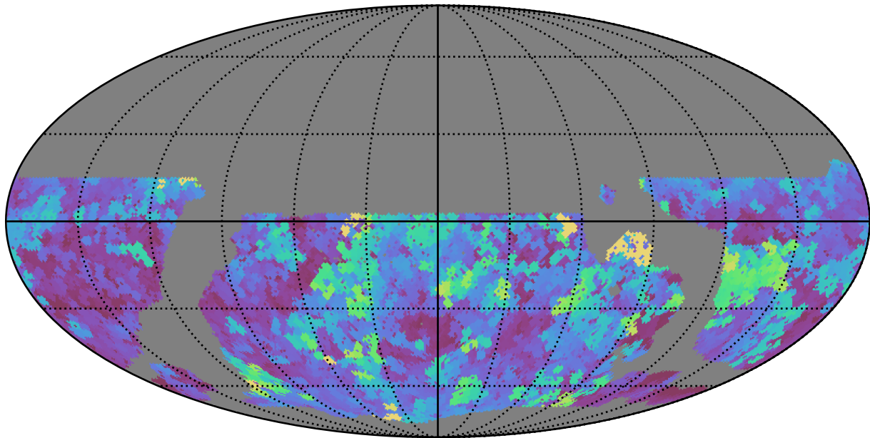
weather_cloudso31v3.4_10yrs WFD u band: Max seeingEff
