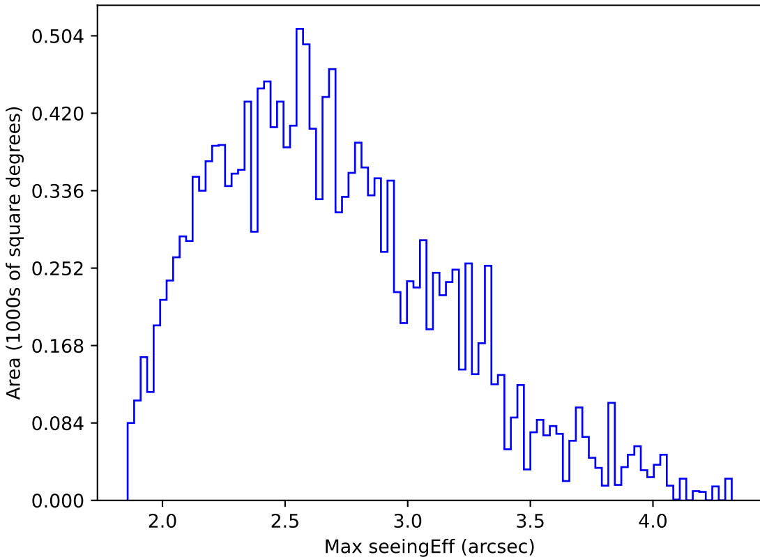
weather_cloudso31v3.4_10yrs WFD u band: Max seeingEff
