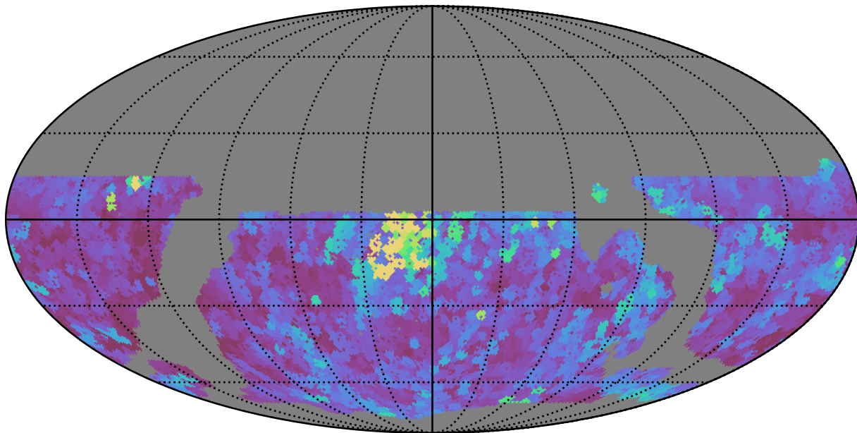
weather_cloudso31v3.4_10yrs WFD r band: Max seeingEff
