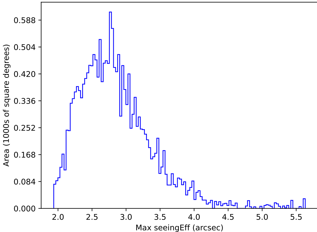
weather_cloudso31v3.4_10yrs WFD r band: Max seeingEff
