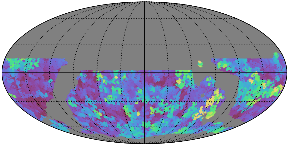
weather_cloudso31v3.4_10yrs WFD g band: Max seeingEff
