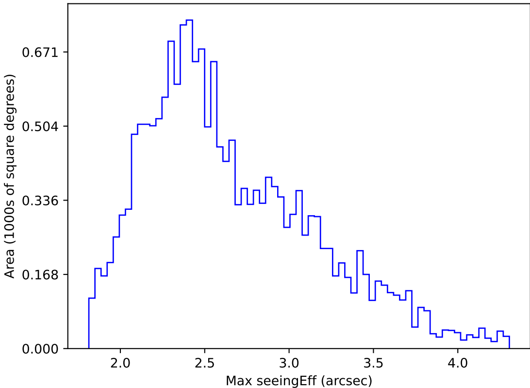
weather_cloudso31v3.4_10yrs WFD g band: Max seeingEff
