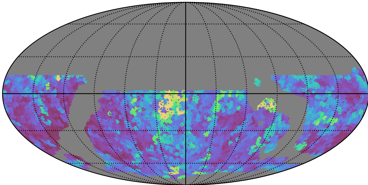
weather_cloudso31v3.4_10yrs WFD all bands: Max seeingEff
