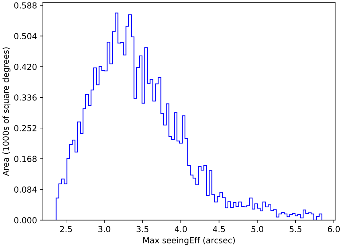
weather_cloudso31v3.4_10yrs WFD all bands: Max seeingEff
