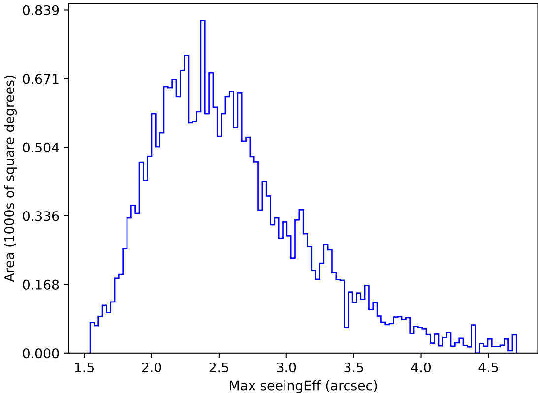
weather_cloudso31v3.4_10yrs All sky z band: Max seeingEff
