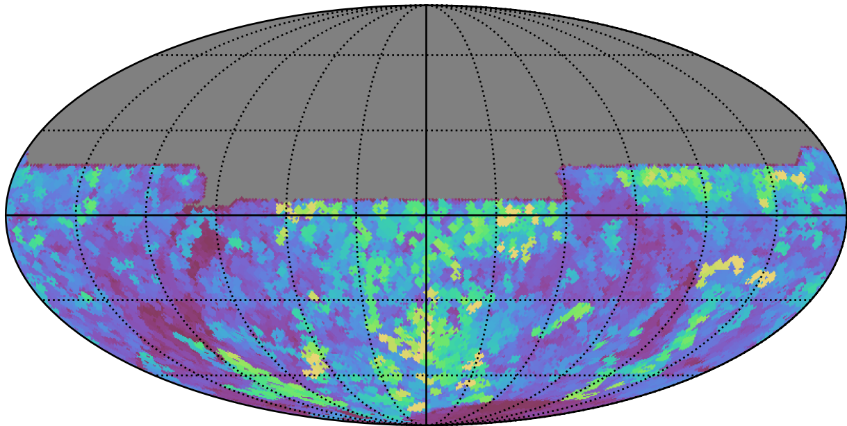
weather_cloudso31v3.4_10yrs All sky y band: Max seeingEff
