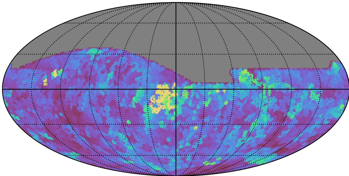
weather_cloudso31v3.4_10yrs All sky r band: Max seeingEff
