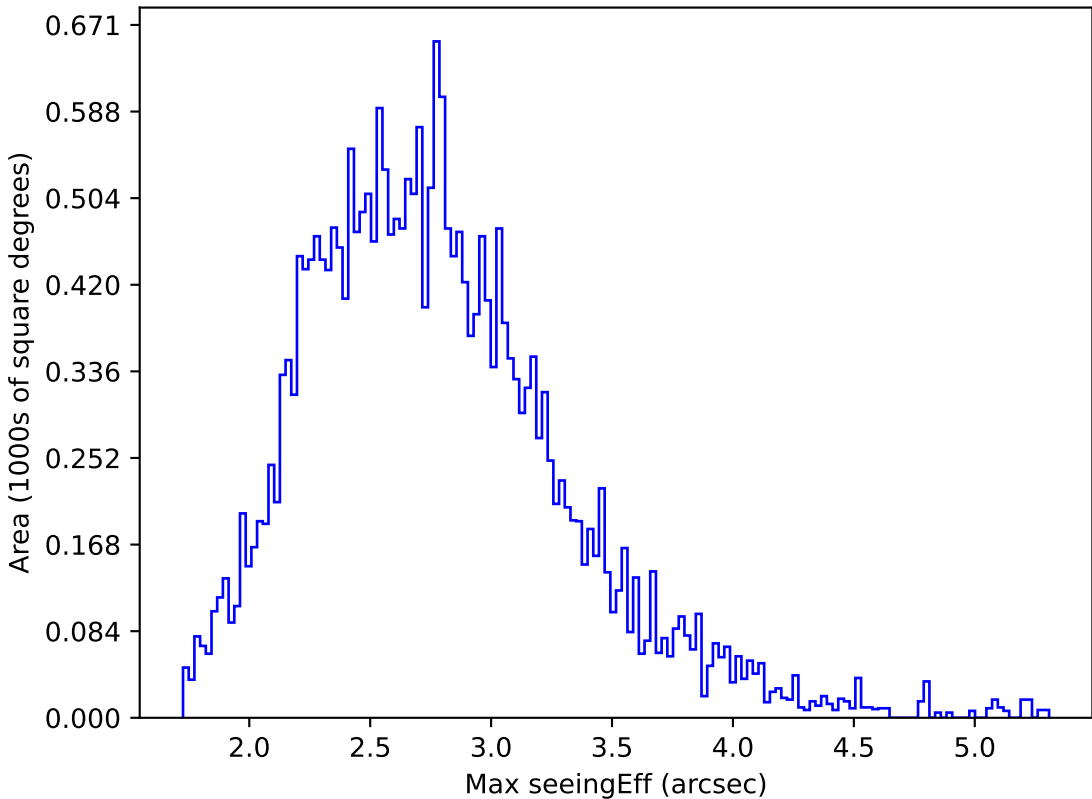
weather_cloudso31v3.4_10yrs All sky r band: Max seeingEff
