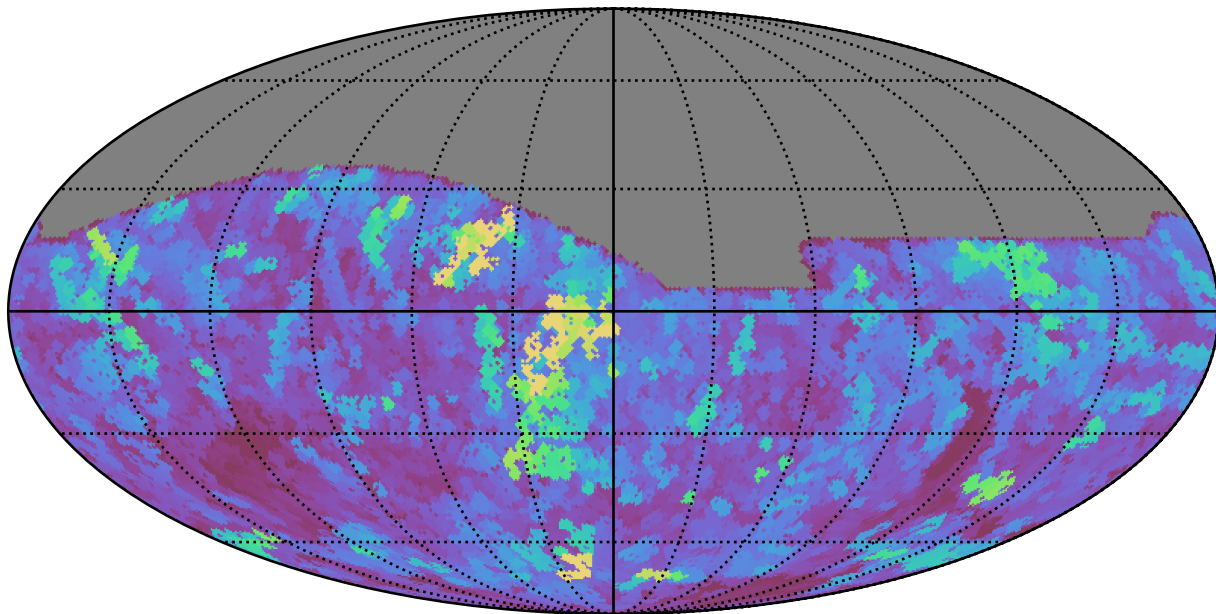
weather_cloudso31v3.4_10yrs All sky i band: Max seeingEff
