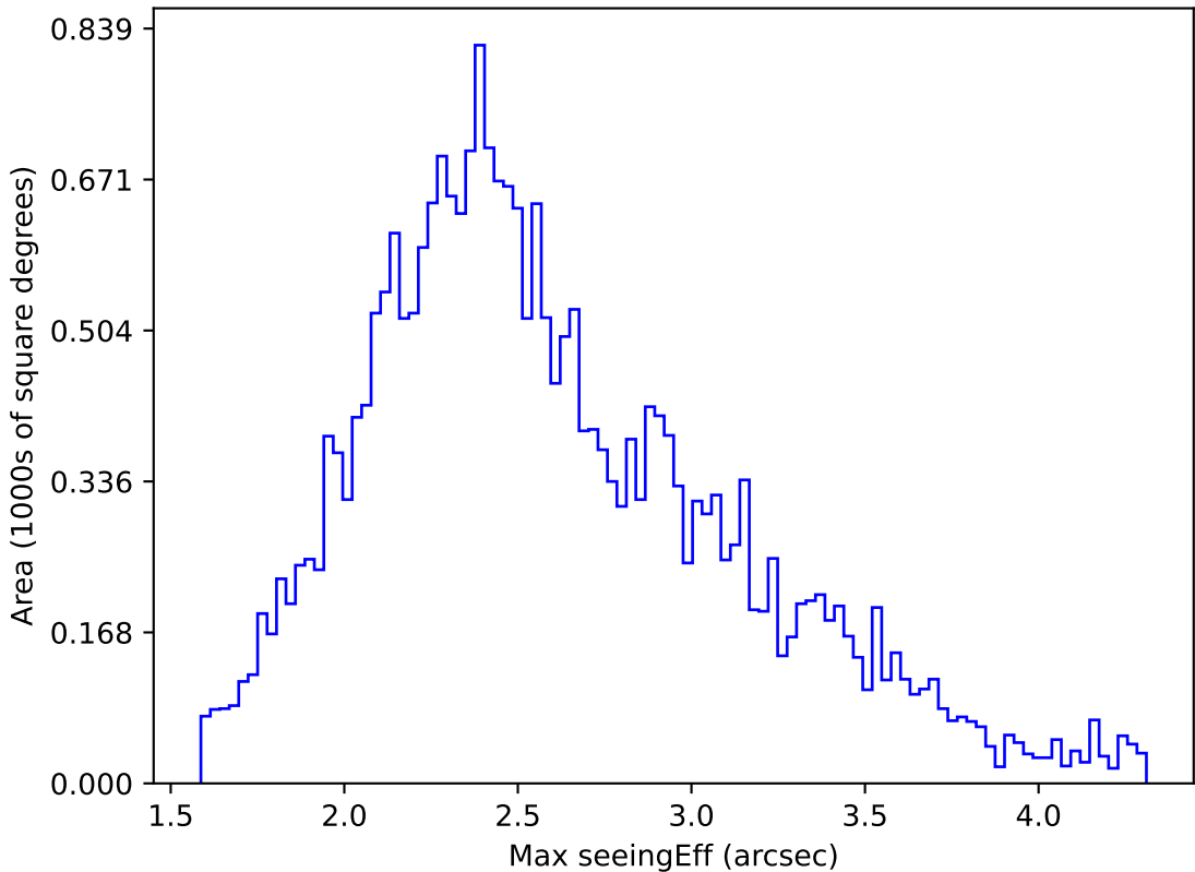
weather_cloudso31v3.4_10yrs All sky g band: Max seeingEff
