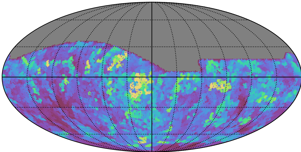
weather_cloudso31v3.4_10yrs All sky all bands: Max seeingEff
