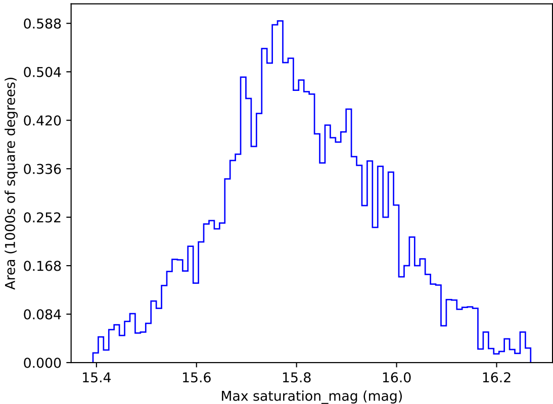
weather_cloudso31v3.4_10yrs WFD all bands: Max saturation_mag
