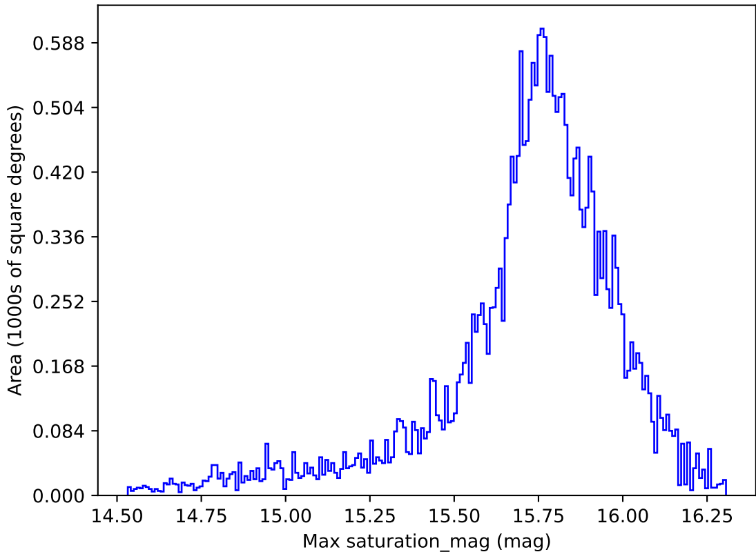
weather_cloudso31v3.4_10yrs All sky all bands: Max saturation_mag
