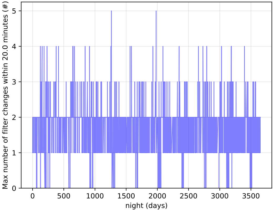
weather_cloudso31v3.4_10yrs Per Night: Max number of filter changes within 20.0 minutes
