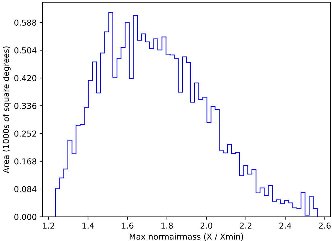
weather_cloudso31v3.4_10yrs WFD u band: Max normairmass
