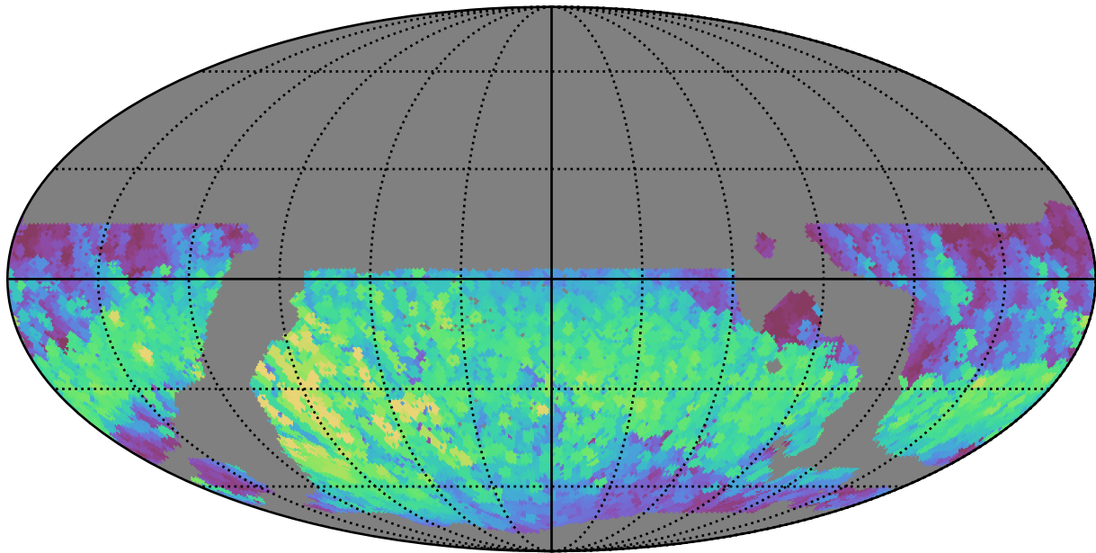
weather_cloudso31v3.4_10yrs WFD r band: Max normairmass
