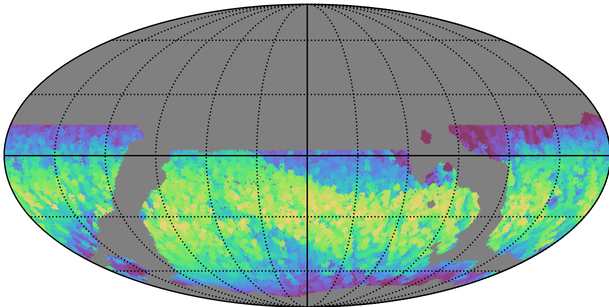
weather_cloudso31v3.4_10yrs WFD all bands: Max normairmass
