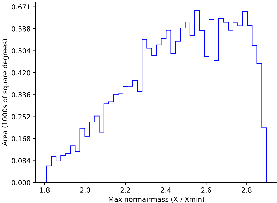
weather_cloudso31v3.4_10yrs WFD all bands: Max normairmass
