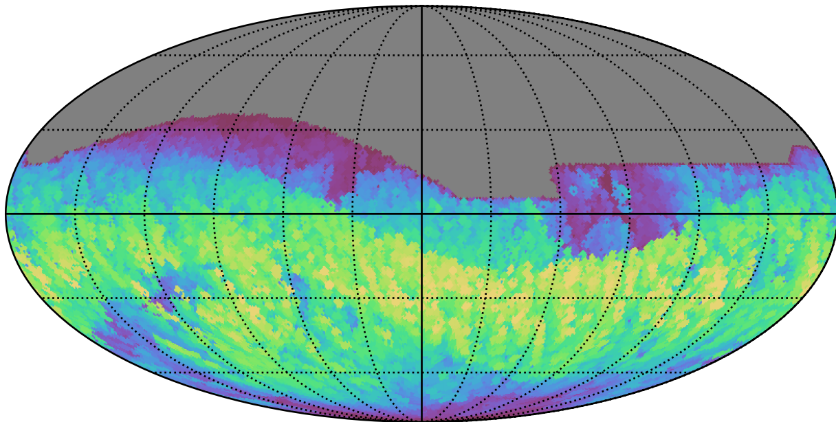
weather_cloudso31v3.4_10yrs All sky z band: Max normairmass
