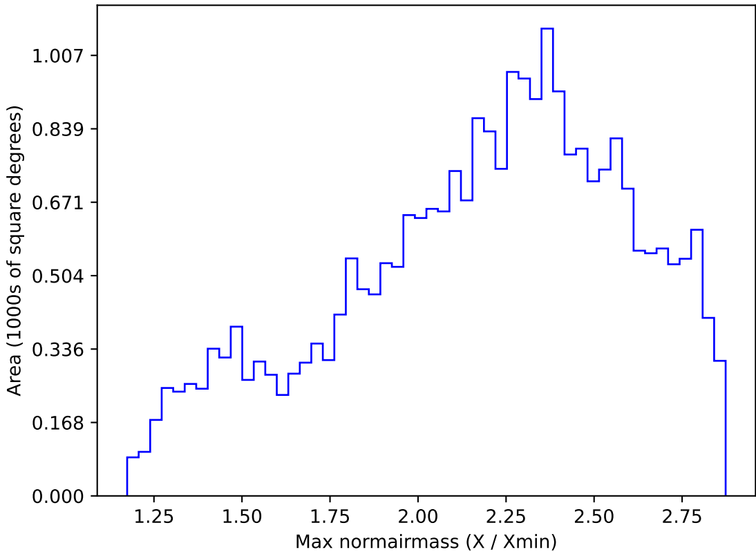
weather_cloudso31v3.4_10yrs All sky z band: Max normairmass
