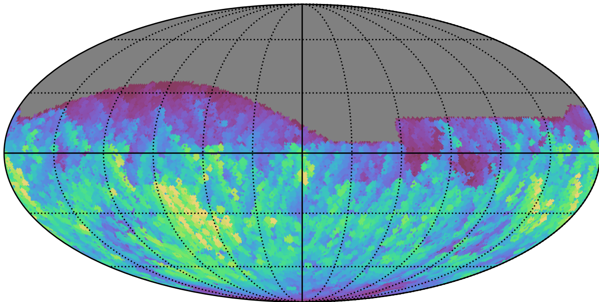
weather_cloudso31v3.4_10yrs All sky g band: Max normairmass
