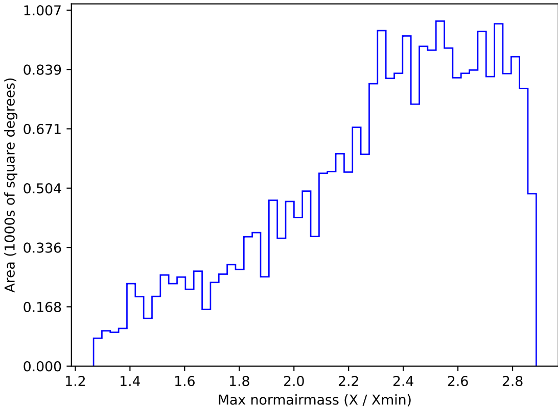
weather_cloudso31v3.4_10yrs All sky all bands: Max normairmass
