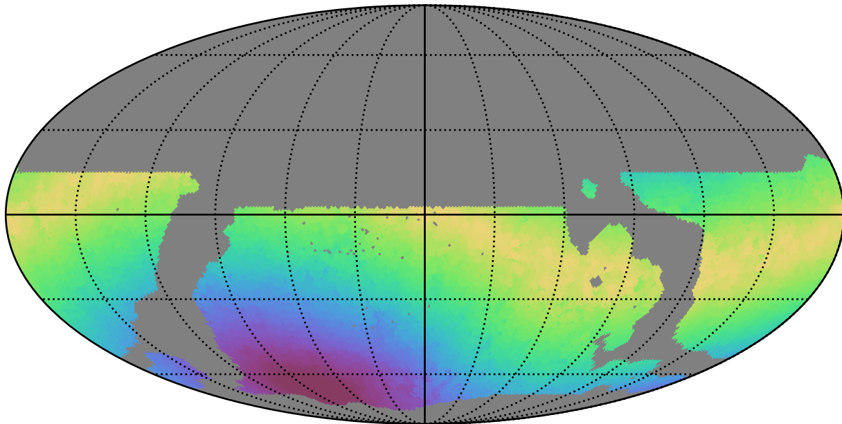
weather_cloudso31v3.4_10yrs WFD z band: Max moonDistance
