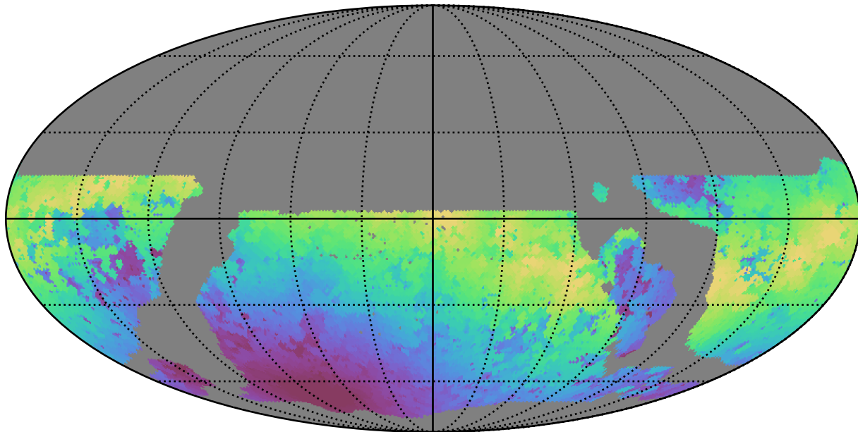
weather_cloudso31v3.4_10yrs WFD y band: Max moonDistance
