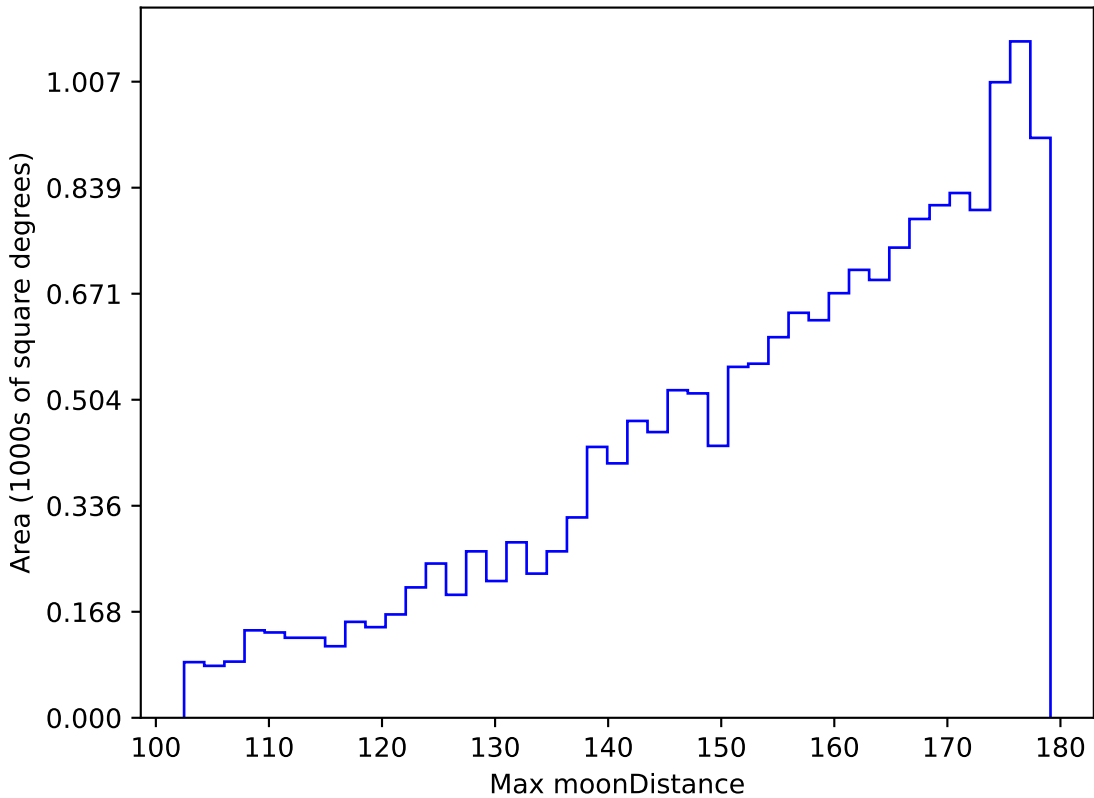
weather_cloudso31v3.4_10yrs WFD u band: Max moonDistance
