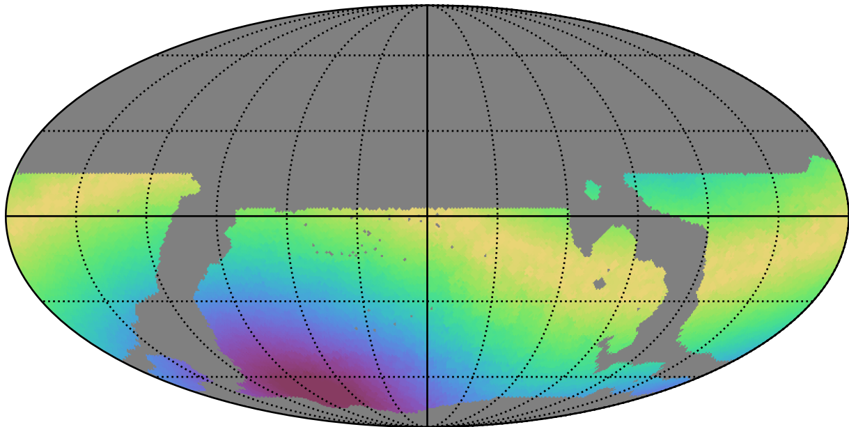
weather_cloudso31v3.4_10yrs WFD r band: Max moonDistance
