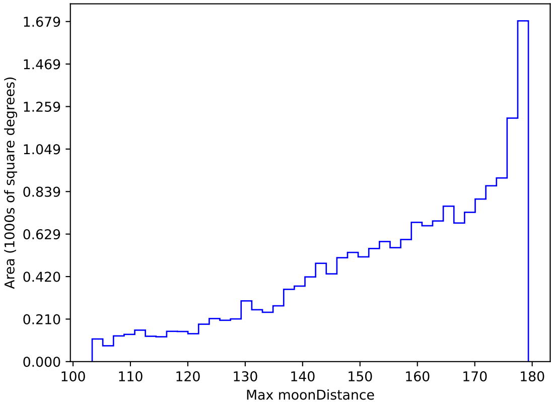
weather_cloudso31v3.4_10yrs WFD r band: Max moonDistance
