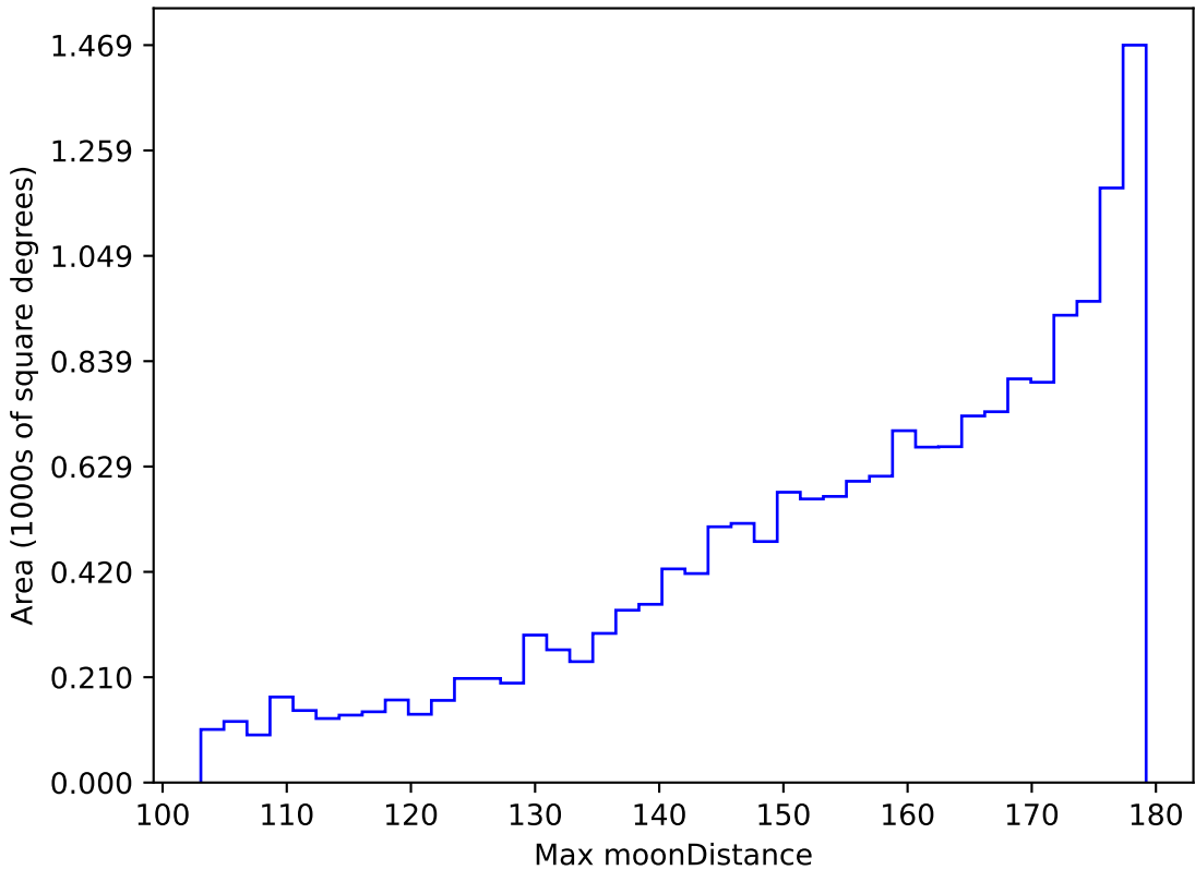
weather_cloudso31v3.4_10yrs WFD i band: Max moonDistance
