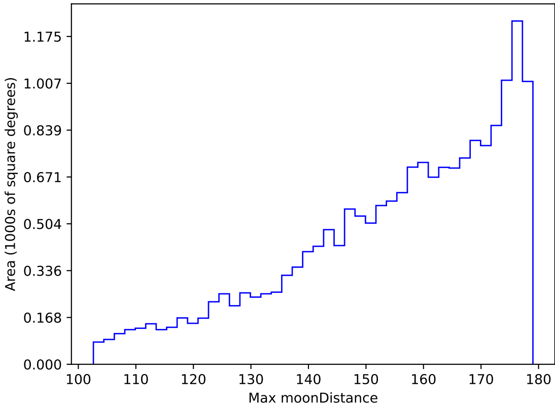
weather_cloudso31v3.4_10yrs WFD g band: Max moonDistance
