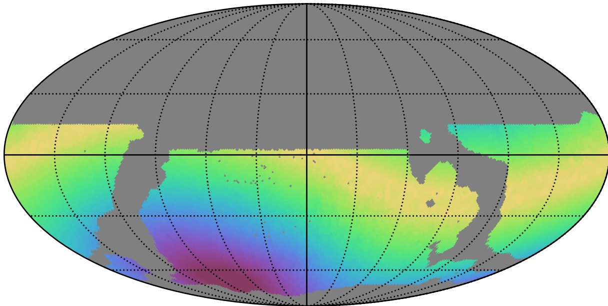
weather_cloudso31v3.4_10yrs WFD all bands: Max moonDistance
