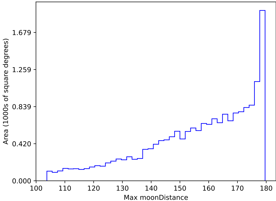
weather_cloudso31v3.4_10yrs WFD all bands: Max moonDistance
