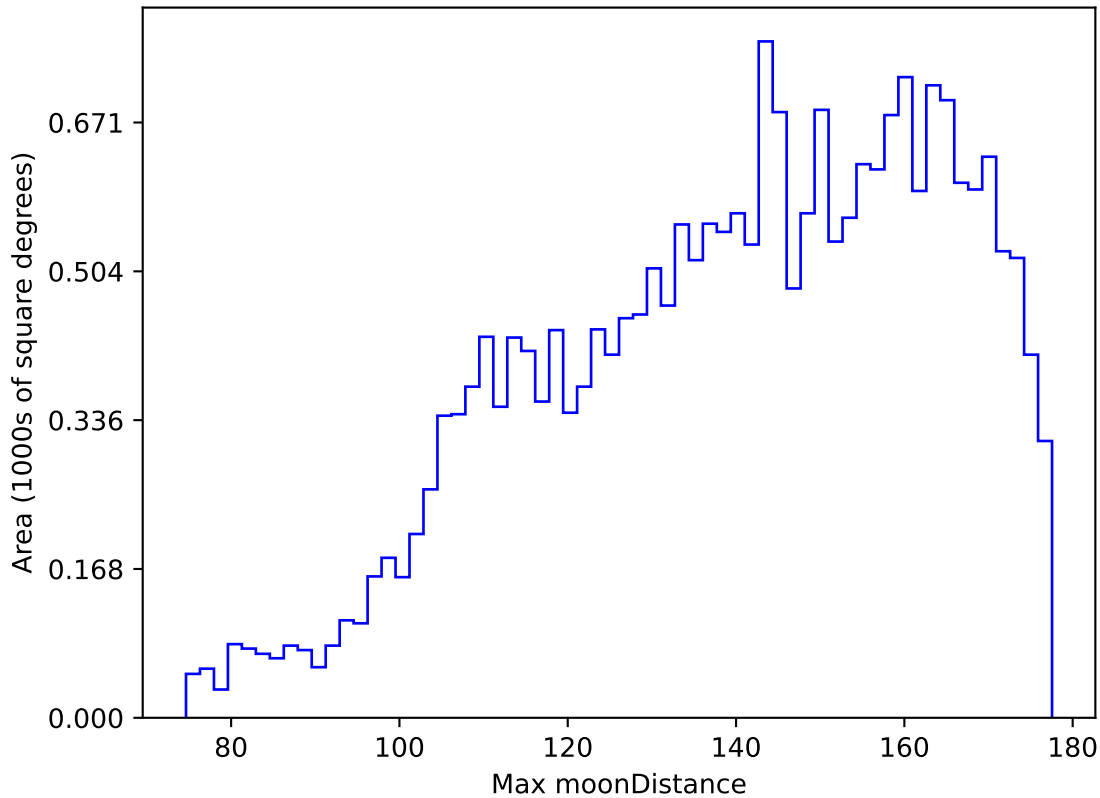
weather_cloudso31v3.4_10yrs All sky y band: Max moonDistance
