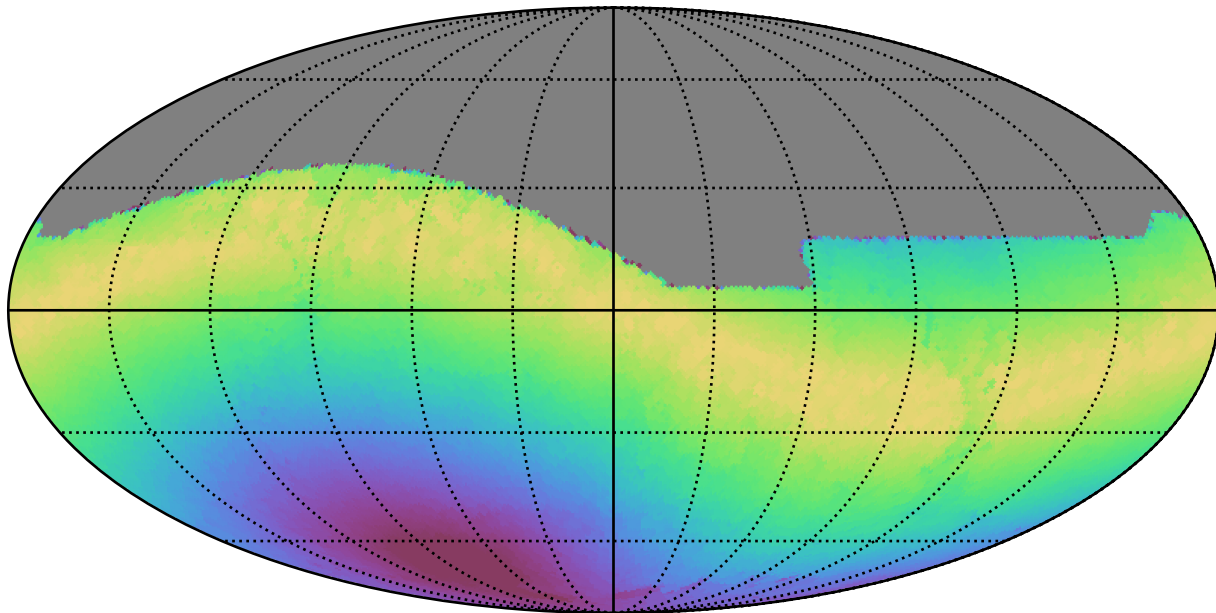
weather_cloudso31v3.4_10yrs All sky r band: Max moonDistance
