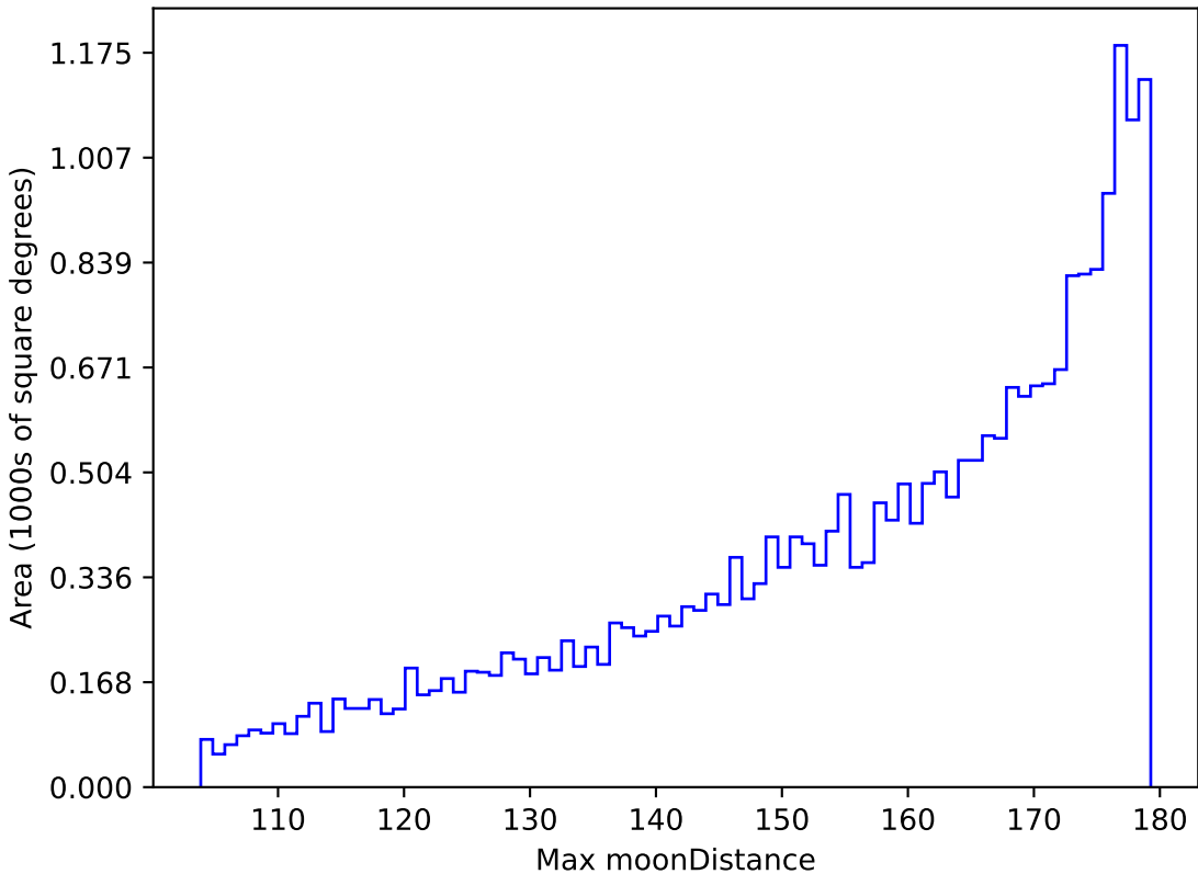
weather_cloudso31v3.4_10yrs All sky r band: Max moonDistance
