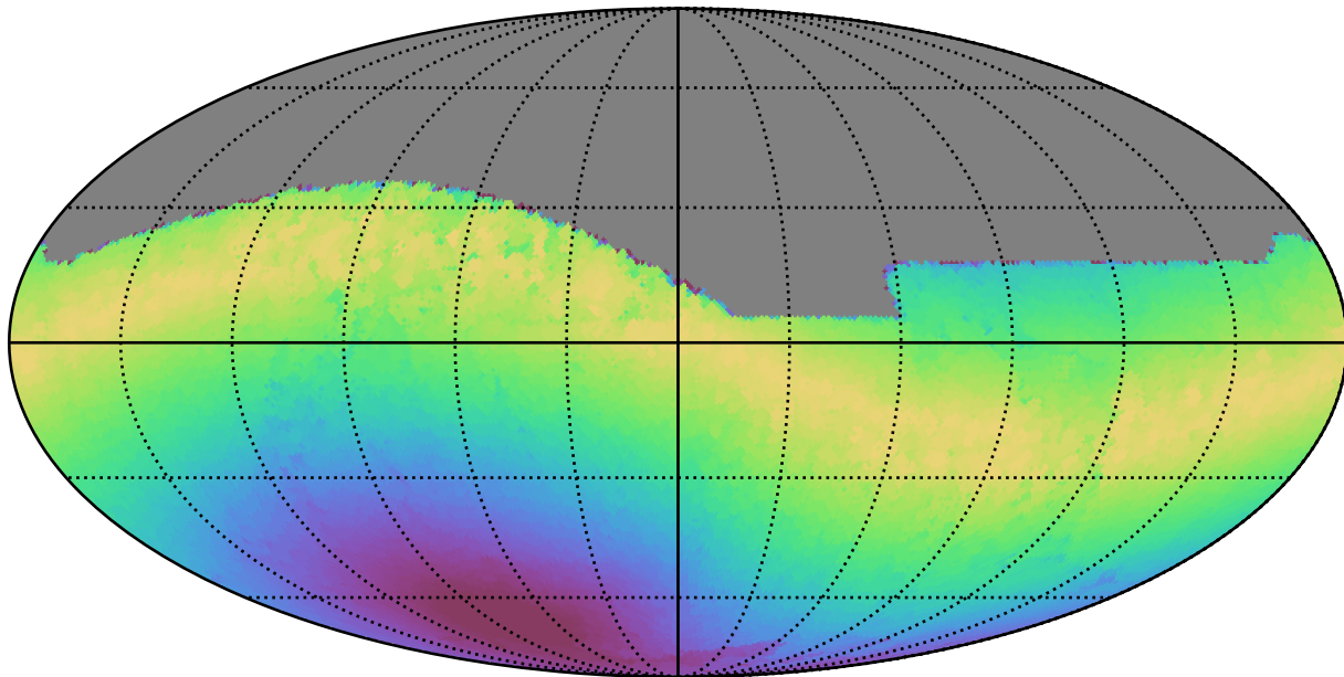
weather_cloudso31v3.4_10yrs All sky i band: Max moonDistance
