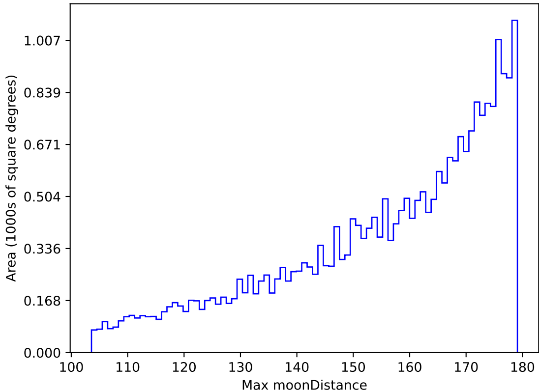
weather_cloudso31v3.4_10yrs All sky i band: Max moonDistance
